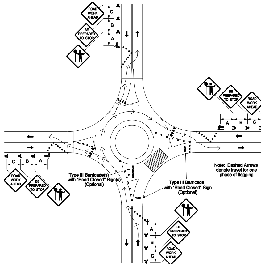
Sign Spacing and Buffer Lengths (feet)
