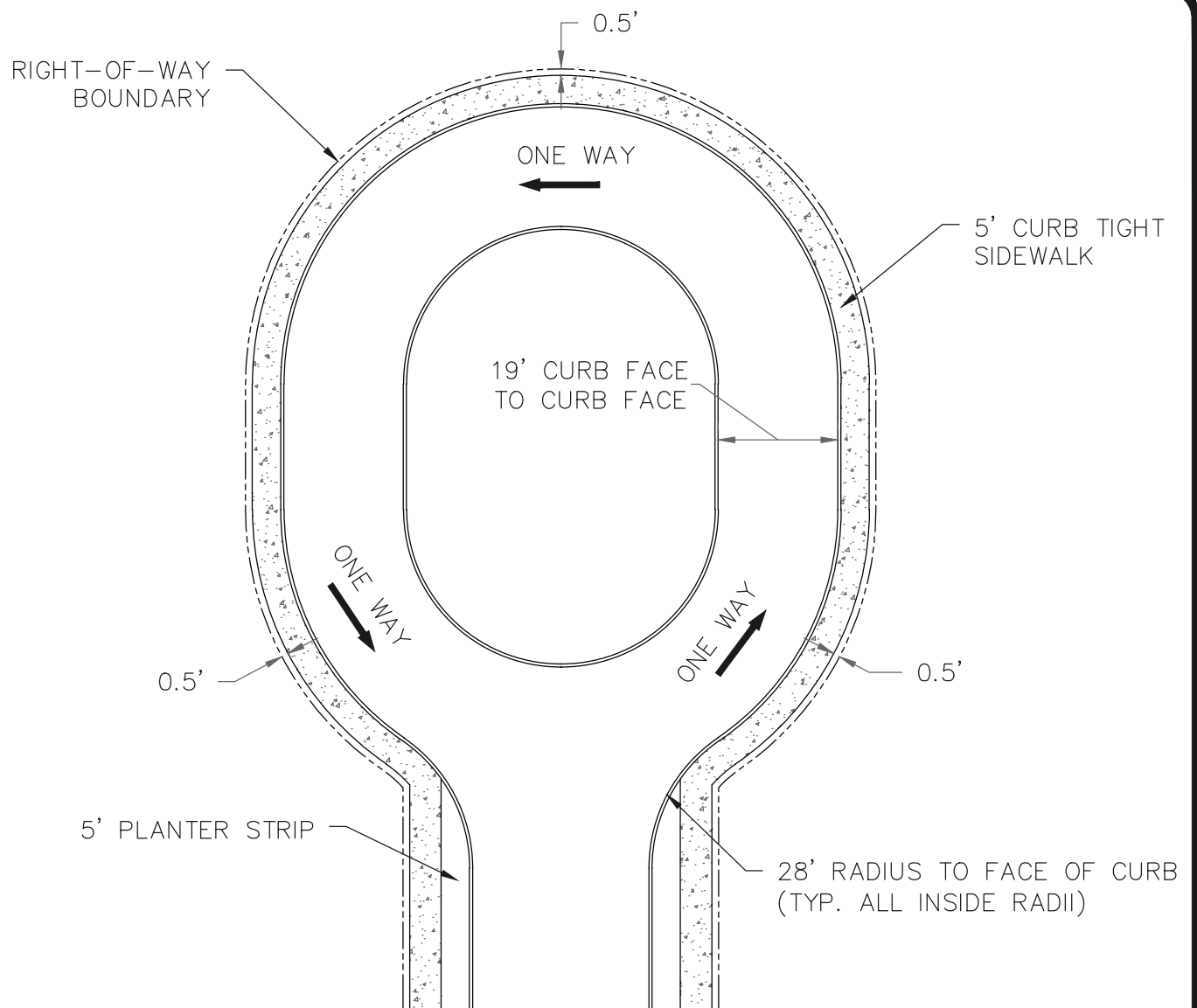
LOOP TURN-AROUND (PLAN VIEW) SCALE = N.T.S.
